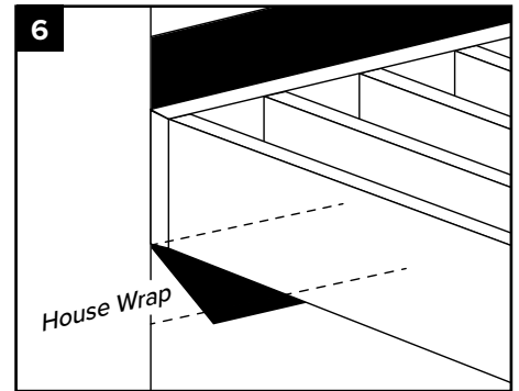
6. Install the house wrap and slide it up behind the remaining section of the sub-ledger tape. Then peel off the remaining release liner and smooth the tape over the house wrap.
