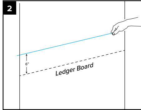
2. Measure up 6" and snap a chalk line the width of the deck.
